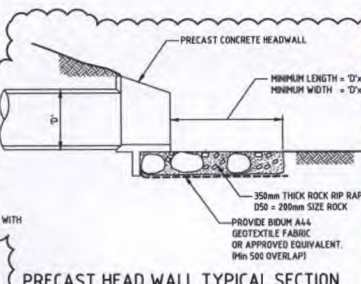
PRECAST HEAD WALL TYPICAL SECTION
