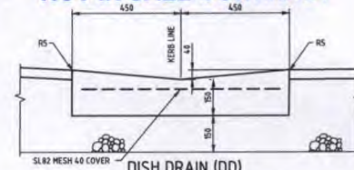
DISH DRAIN (DD)
