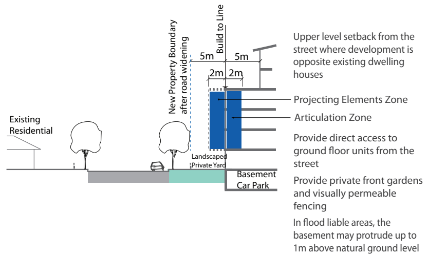
Street Section
