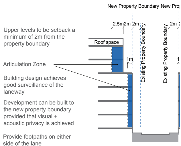
Section: Lane Frontage
