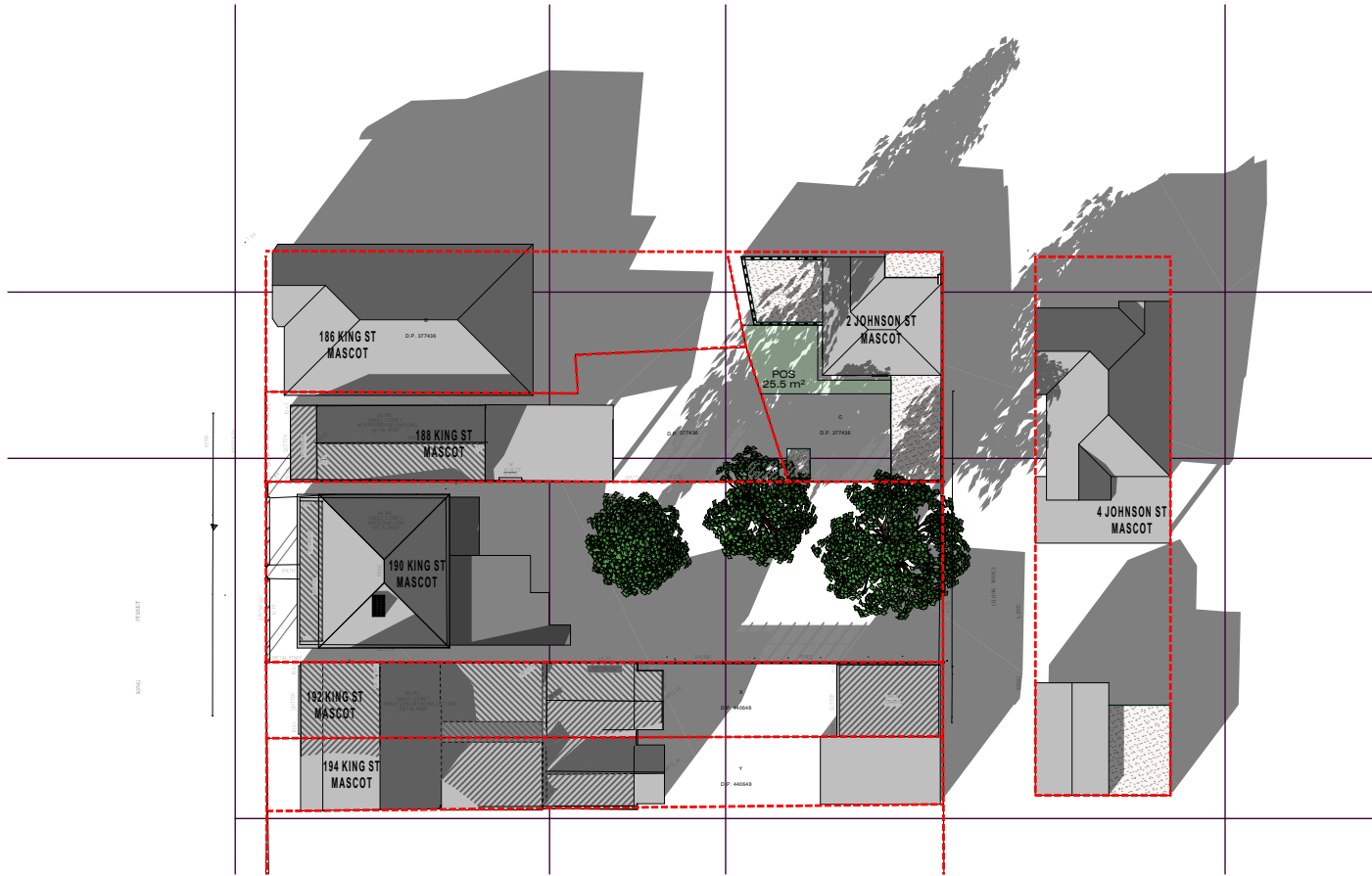
1 EXISTING JUNE 1500 (1) 1:500
