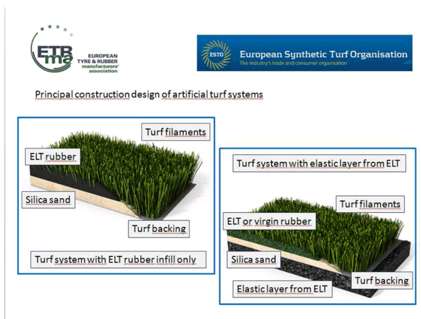
Figure 2.2 Two types of synthetic turf systems
