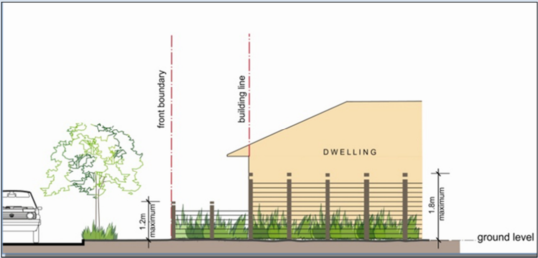
Figure 21 - Side Fences
