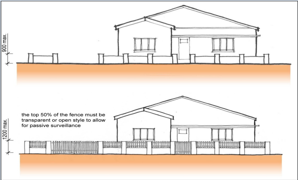
Figure 20 - Front Fences
