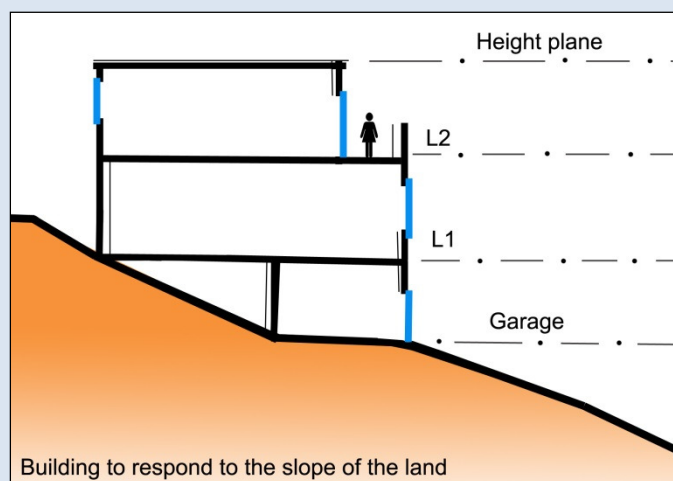
Figure 10 - Three Storey Dwellings are Permitted in Special Area H3 1
