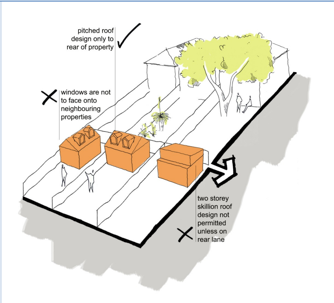
Figure 28 - Ancillary Development in Lot-to-Lot context.
