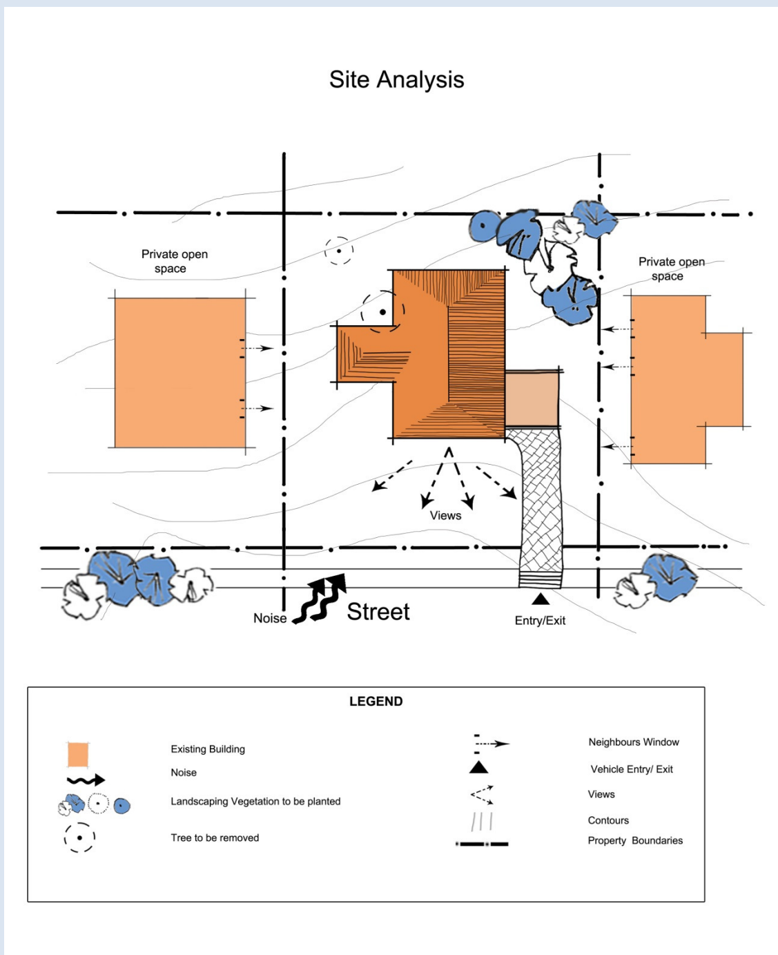
Figure 1 - Example of a Site Analysis Plan
