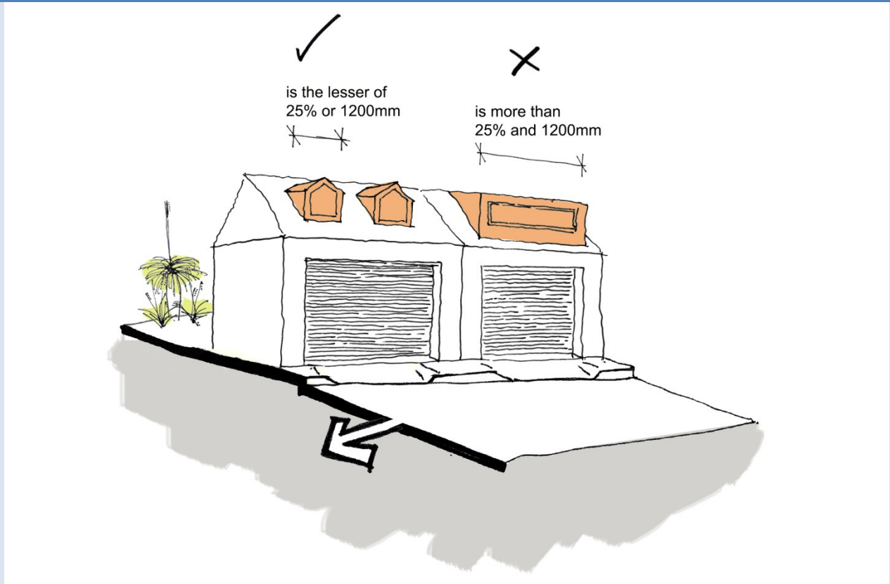
Figure 27 - A dormer is to be the lesser of 25% of the roof width, or 1200mm.
