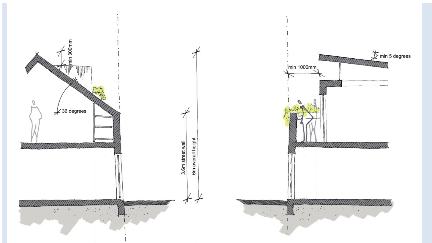
Figure 29 - Section through rear lane showing potential envelopes.
